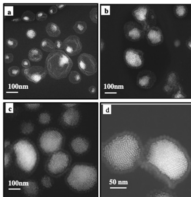
Fig. 5 2D HAADF-STEM (a)–(d) overview of superstructures of 10 nm Fe 3 O 4 nanocrystals (2 mg mL -1 ) and 5 nm Au nanocrystals differing by their amounts: (a) 10 mg mL -1 , (b) 60 mg mL -1 , (c) 100 mg mL -1 and (d) 200 mg mL -1 .
