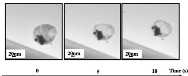
Fig. 4 "Egg" suprastructures of 4 mg mL -1 of Fe 3 O 4 NCs and 0.3 mg mL -1 of Au NCs dispersed in an aqueous solution. The electron dose is around 1.69 \times 10^{14} e nm -2 s -1 .
