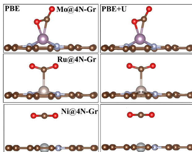
Fig. 3 \text{CO}_2 adsorption on \text{TM}@4\text{N-Gr} : chemisorption versus physisorption. Left: PBE; right: PBE+U.
