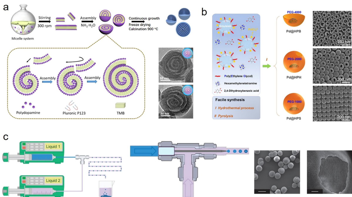
Fig. 2 Schematic illustration of various bottom-up methods and transmission electron microscopy images of corresponding hollow nanomaterials: (a) micelle-directed assembly, 20 Copyright 2021, Science; (b) emulsion-guided assembly, 24 Copyright 2023, American Chemical Society; and (c) interfacial assembly methods, 25 Copyright 2011, Nature Publishing Group.
