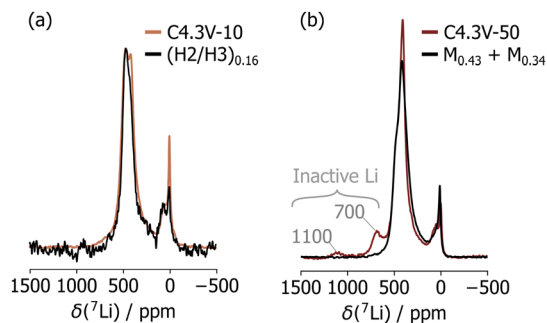
Fig. 4 (a) Comparison of the {}^7\text{Li} NMR spectrum collected on C4.3V-10 and the first cycle spectrum for (\text{H2}/\text{H3})_{0.16} . (b) Comparison of the {}^7\text{Li} NMR spectrum collected on C4.3V-50 with the sum of spectra acquired on \text{M}_{0.43} and \text{M}_{0.34} . The spectra collected on the \text{M}_{0.43} and \text{M}_{0.34} were scaled \text{M}_{0.43} : \text{M}_{0.34} = 1 : 3.8 .
