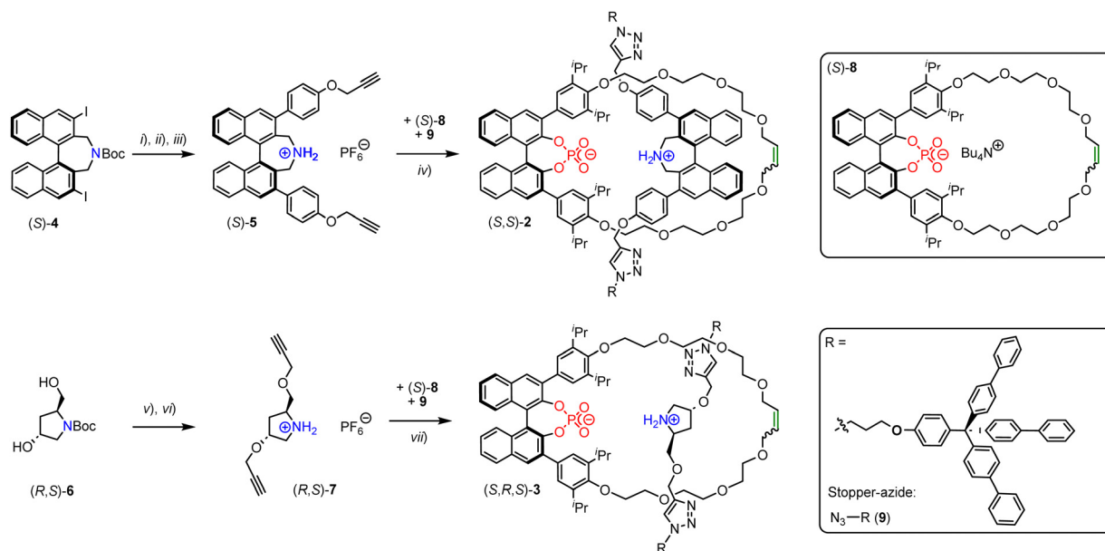
Fig. 2 Synthesis of rotaxanes (S,S)-2 and (S,R,S)-3. Reagents and conditions: (i) 4-hydroxyphenylboronic acid, \text{Pd}(\text{PPh}_3)_4 , 2 M \text{Na}_2\text{CO}_3 (aq.), DME, 90 °C, 2 h, 81%; (ii) propargyl bromide, cesium carbonate, DMF, 1.5 h, 68% (iii) trifluoroacetic acid, DCM, r.t., 2 h, then NaOH, then hydrochloric acid/dioxane, \text{Et}_2\text{O} , r.t., 30 min, then ammonium hexafluorophosphate, DCM, r.t., 16 h, 81%; (iv) [\text{Cu}(\text{MeCN})_4\text{PF}_6] , \text{CH}_2\text{Cl}_2 , r.t., 4 h, 20%; (v) propargyl bromide, sodium hydride, THF, r.t. 16 h, 70%; (vi), trifluoroacetic acid, DCM, r.t., 16 h, then NaOH, then hydrochloric acid/dioxane, \text{Et}_2\text{O} , r.t., 30 min, then ammonium hexafluorophosphate, DCM, r.t., 16 h, 79%; (vii) [\text{Cu}(\text{MeCN})_4\text{PF}_6] , \text{CH}_2\text{Cl}_2 , r.t., 4 h, 37%.
