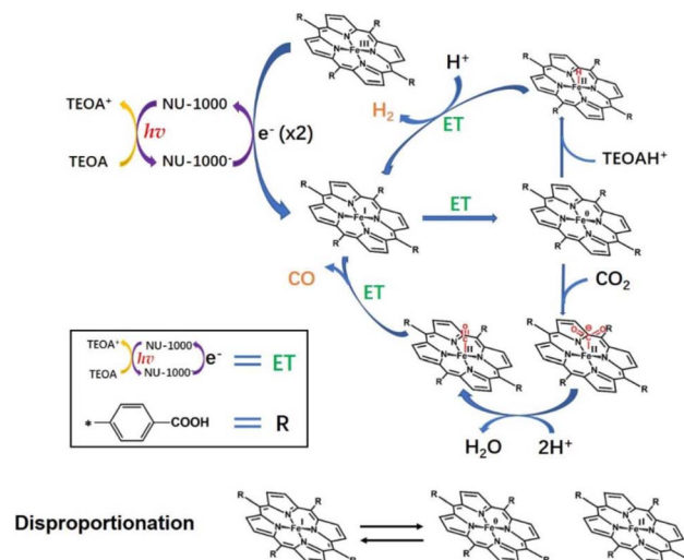
Scheme 9 Proposed mechanism for photocatalytic reduction of \text{CO}_2 using an \text{Fe-TCPP@NU-1000} heterogeneous catalyst with TEOA as a sacrificial agent. Reprinted from ref. 90 with permission from Elsevier (Copyright 2022).
