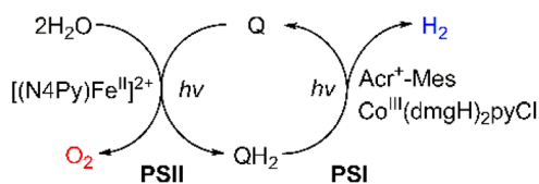
Scheme 18 Schematic diagram of light-driven H 2 O splitting with the combination of PSI and PSII models. Reprinted from ref. 159 with permission from American Chemical Society (Copyright 2022).
