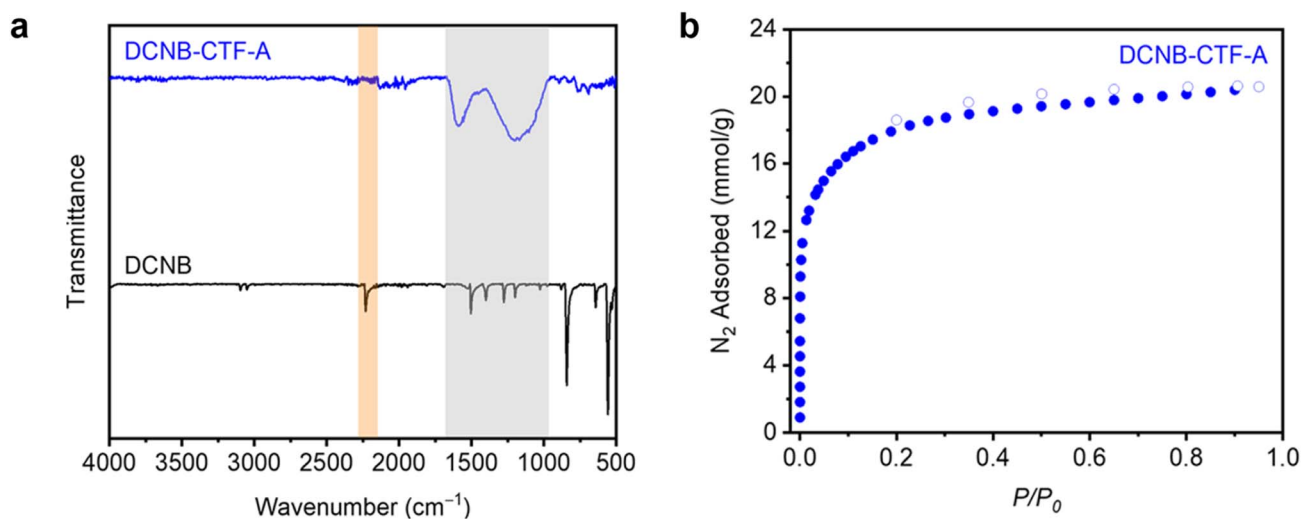
Fig. 6 Solid-state characterization of DCNB-CTF-A made with 5.00 equiv. of \text{ZnBr}_2 at 400 \text{ }^\circ\text{C} for 40 h. (a) ATR-IR spectra of DCNB and DCNB-CTF-A . The orange highlighted region shows the disappearance of the \text{C}\equiv\text{N} stretch from DCNB , and the gray highlighted region indicates the appearance of triazine stretches in DCNB-CTF-A . (b) 77 K \text{N}_2 adsorption (filled circles) and desorption (open circles) isotherms of DCNB-CTF-A .
