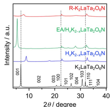
Fig. 1 XRD patterns obtained from the \text{K}_2\text{LaTa}_2\text{O}_6\text{N} and its derivatives.
