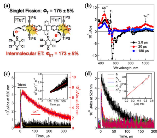
Fig. 18 (a) Schematic diagram of intermolecular electron transfer from iSF of tetracene dimer 14 to chloranil. (b) \mu\text{s} -TA spectra of dimer 14 ( 50 \mu\text{M} ) in the presence of 250 \mu\text{M} chloranil in Ar-saturated PhCN after excitation at 532 \text{ nm} . (c) Time profiles of absorption at 520 \text{ nm} in the presence of different concentrations of chloranil: (a) 0 \text{ mM} , (b) 0.25 \text{ mM} , (c) 0.53 \text{ mM} , (d) 0.63 \text{ mM} , and (e) 0.72 \text{ mM} . The inset shows the plot of the pseudo-first-order rate constant ( k_{\text{obs}} ) vs. the concentration of chloranil. Reproduced with permission. 75 Copyright 2019, the American Chemical Society.
