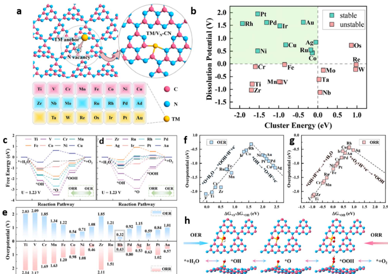
Fig. 32 (a) Schematic representation of various transition metals (TM) based SACs on VN-CN, (b) stability of TM/ \text{V}_N -CN based on cluster energy ( E_{\text{Clust}} < 0 \text{ eV} ) and dissolution potential ( U_{\text{diss}} > 0 \text{ eV} ), the free energy diagrams of TM/ \text{V}_N -CN (c) from Ti to Cu and (d) from Zr to Au related to both OER and ORR at the equilibrium potential of 1.23 V, (e) The OER and ORR overpotentials of TM/ \text{V}_N -CN (from Ti to Au), the volcano plots of (f) OER ( -\eta_{\text{OER}} vs. \Delta G^*\text{O} - \Delta G^*\text{OH} ) and (g) ORR ( -\eta_{\text{ORR}} vs. \Delta G^*\text{OH} ) on TM/ \text{V}_N -CN, (h) OER and ORR intermediate structures adsorbed on Rh/ \text{V}_N -CN. Reproduced with permission from ref. 10. Copyright 2021 American Chemical Society.
