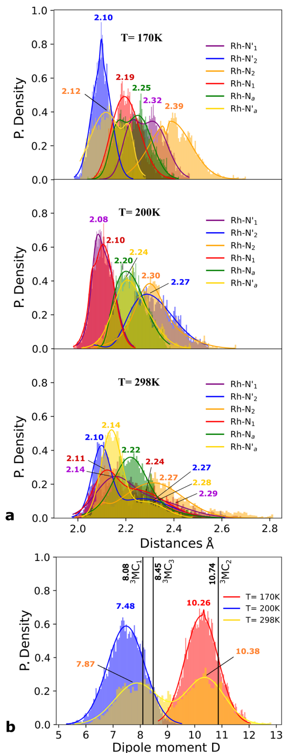
Fig. 2 Probability distributions (P. density) (a) bond distance in Å for the six metal-ligand bonds in the ^3\text{MC} state of the [\text{Rh(III)(phen)}_2(\text{NH}_3)_2]^{3+} complex: Rh-N' 1 (purple) and Rh-N' 2 (blue) in phen', Rh-N 1 (red) and Rh-N 2 (orange) in phen, and Rh-N' a (yellow) and Rh-N a (green) during a 7.5 ps AIMD sampling at 170 K, 200 K, and 298 K. (b) Dipole moment in D for the ^3\text{MC} state in the [\text{Rh(III)(phen)}_2(\text{NH}_3)_2]^{3+} complex for 7.5 ps AIMD sampling at (red) 170 K, (blue) 200 K, (yellow) 298 K. Vertical black lines mark the calculated dipole moment in D at the uDFT minimized structures for the ^3\text{M}_1 , ^3\text{MC}_2 , and ^3\text{MC}_3 excited states.
