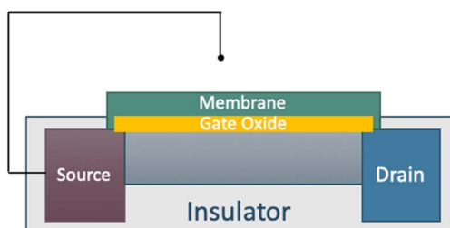
Fig. 1 Chemically sensitive field effect transistor (ChemFET) diagram. For sensor construction, pre-constructed FETs are covered with insulating epoxy, except for the gate nitride/oxide surface, which is coated with the ionophore-containing membranes. Reference electrodes are constructed separately.
