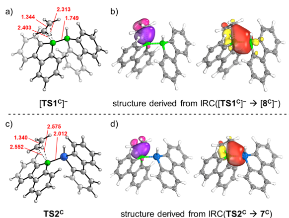
Fig. 2 (a) Computed geometry of [TS1^C]^- . (b) Two IBOs observed on a structure at 2.582 bohr amu^{1/2} along the IRC( [TS1^C]^- \rightarrow [8^C]^- ) path; IBO contributions: left: C(dist) = 0.77, C(prox) = 0.76, prev. B(sp 2 ) = 0.43, others = 0.04; right: C(dist) = 0.08, C(prox) = 0.11, prev. B(sp 2 ) = 0.90, B(sp 3 ) = 0.74, others = 0.17. (c) Computed geometry of TS2^C . (d) Two IBOs observed on a structure at 15.076 bohr amu^{1/2} along the IRC( TS2^C \rightarrow 7^C ) path; IBO contributions: left: C(dist) = 0.76, C(prox) = 0.65, prev. B(sp 2 ) = 0.55, others = 0.04; right: C(dist) = 0.10, C(prox) = 0.17, prev. B(sp 2 ) = 0.92, Si(sp 3 ) = 0.72, others = 0.08. Highlighted in red are selected bond lengths and atom...atom distances (in Å). Prox, dist: proximal, distal with respect to the B...E core; prev. = previously.
