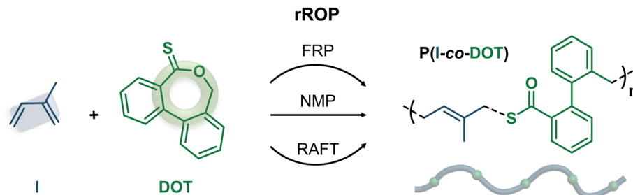
Fig. 2 Synthesis of poly(isoprene-co-dibenzoc[e]oxepane-5-thione) (P(I-co-DOT)) copolymers by radical ring-opening copolymerization (rROP) of DOT and I in dioxane at 115 °C by: (a) free-radical polymerization (FRP); (b) nitroxide-mediated polymerization (NMP) and (c) reversible addition-fragmentation chain-transfer (RAFT) polymerization.
