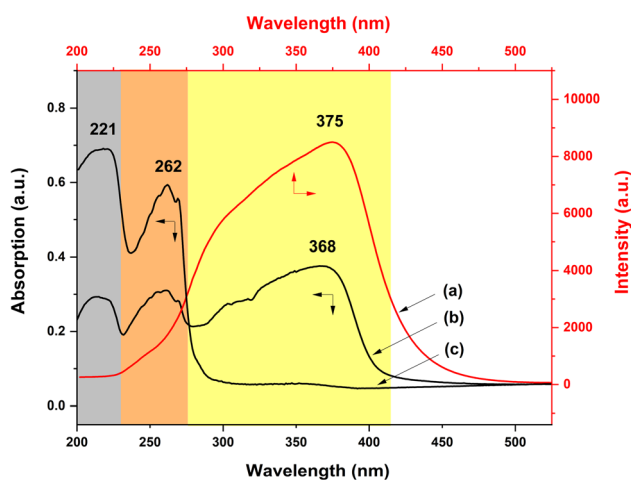
Fig. 9 Excitation (a) and UV-vis absorption (b) spectra of the PS–Eu fiber membrane and UV-vis absorption spectrum (c) of the neat PS fiber membrane.
