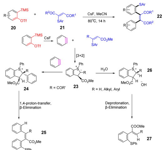
d. Cycloaddition of sulfonium ylides (studer et al.)
