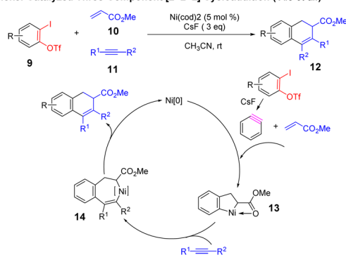
b. Nickel-Catalyzed Three-Component [2+2+2] Cycloaddition (Xie et al.)
