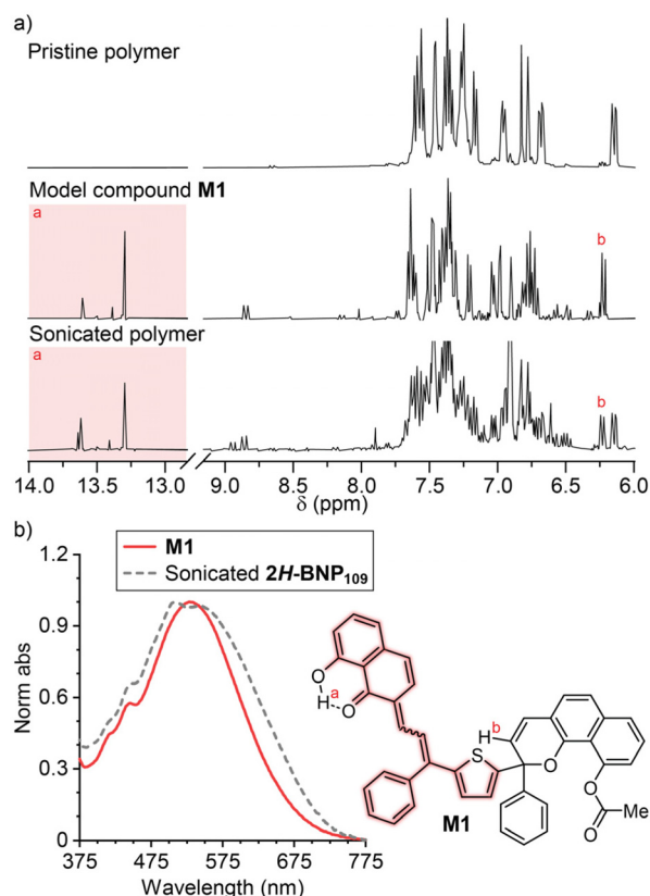
Fig. 3 (a) Characteristic resonances in the ^1\text{H} NMR (THF- d_8 , 400 MHz) spectrum of model compound M1 are also observed in the product mixture generated from ultrasound-mediated mechanical activation of 2H-BNP 109 . (b) The absorption spectrum generated upon ultrasonication of 2H-BNP 109 is bathochromically shifted compared to the absorption spectrum of M1 .
