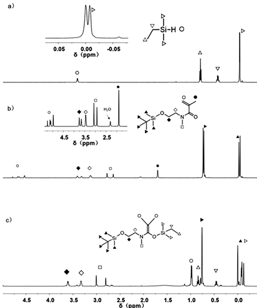
Fig. 1 1 H NMR spectra of (a) Me 2 EtSiH, (b) MAM-TBDMS, and (c) the hydrosilylation product measured in CDCl 3 .
