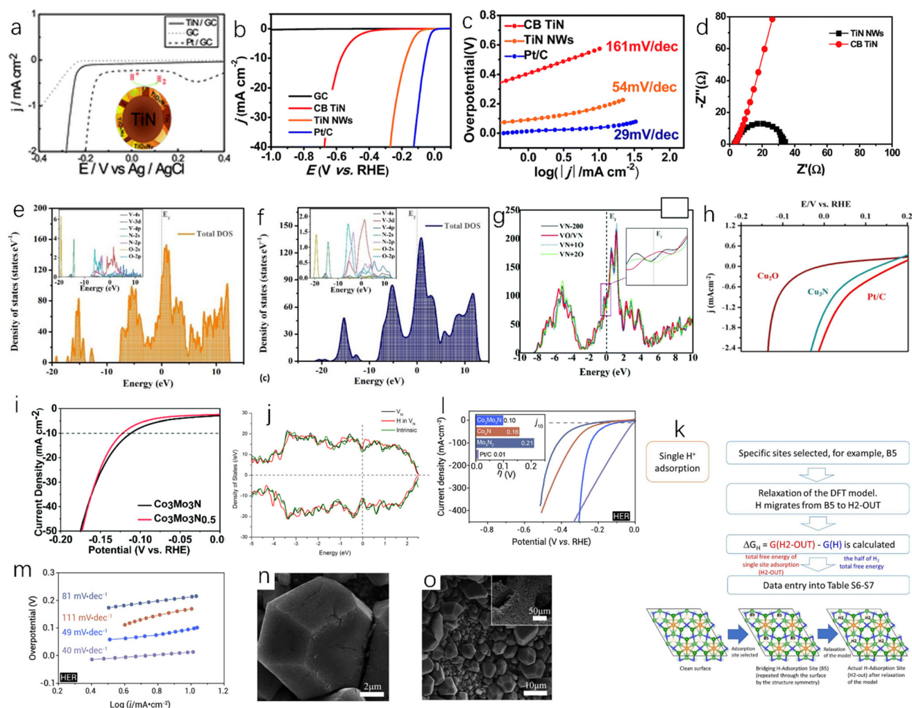
Fig. 6 (a) HER linear sweep voltammograms of GC, TiN-modified GC and Pt-modified GC electrodes in 0.5 M H 2 SO 4 at a scan rate of 5 mV s -1 . Copyright 2012, Royal Society of Chemistry; (b) the polarization curves of TiN NWs electrode in 1 M HClO 4 and CB TiN, commercial Pt/C, bare glassy carbon (GC) electrode in 1 M HClO 4 (after IR correction); (c) Tafel plots corresponding to TiN NW, CB TiN and Pt/C electrodes; (d) Nyquist plots of TiN NWs electrode and CB TiN electrode measured at an overpotential of 0.3 V. 32 Copyright 2016, Royal Society of Chemistry; (e) the density of states of VN (112) surface with single-doped O and (f) double-doped O; (g) comparison of total DOS near the Fermi level of different catalysts. 57 Copyright 2021, Royal Society of Chemistry; (h) the steady-state polarization diagrams of Cu 3 N (160 ml min -1 ammonia flow rate, synthesized at 300 °C), Cu 2 O and Pt/C. 55 Copyright 2022, Springer nature; (i) electrochemical studies of Co 3 Mo 3 N and Co 3 Mo 3 N 0.5 in 0.5 M H 2 SO 4 solution; (j) the total density of states (DOS) of the intrinsic surface (green line), the surface with a N-vacancy (black line), and the surface with a H filled in the N-vacancy (red line); (k) a schematic representation of the algorithm taken to calculate G_{\text{Hads}} for a single site adsorption model. 62 Copyright 2022, Royal Society of Chemistry; (l) comparison of the overpotentials required for the polarization curve (inset) of HER (10 mV s -1 ) to reach 10 mA cm -2 in 1.0 M KOH solution; (m) the corresponding HER Tafel slope. 63 Copyright 2021, ScienceDirect; low (n) and high (o) resolution SEM images of N-NiCoP/NCf. 64 Copyright 2019, ScienceDirect.
