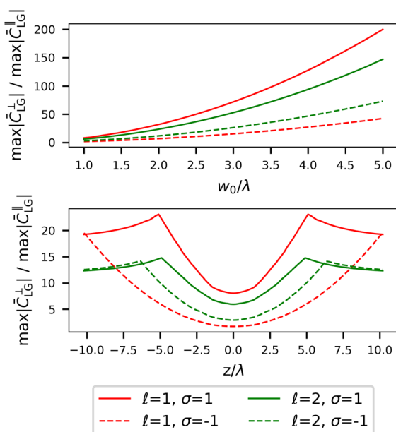
Fig. 7 Ratio of \max|\tilde{C}_{LG}^{\perp}|/\max|\tilde{C}_{LG}^{\parallel}| for p = 1 versus beam waist w_0 (top) and propagation distance from focal plane z = 0 (bottom). The increase in ratio as either the beam waist w_0 or distance from the focal plane increases highlights the rapid decrease in relative magnitude of the longitudinal fields with respect to the transverse fields, i.e. the fields essentially become completely transverse.
