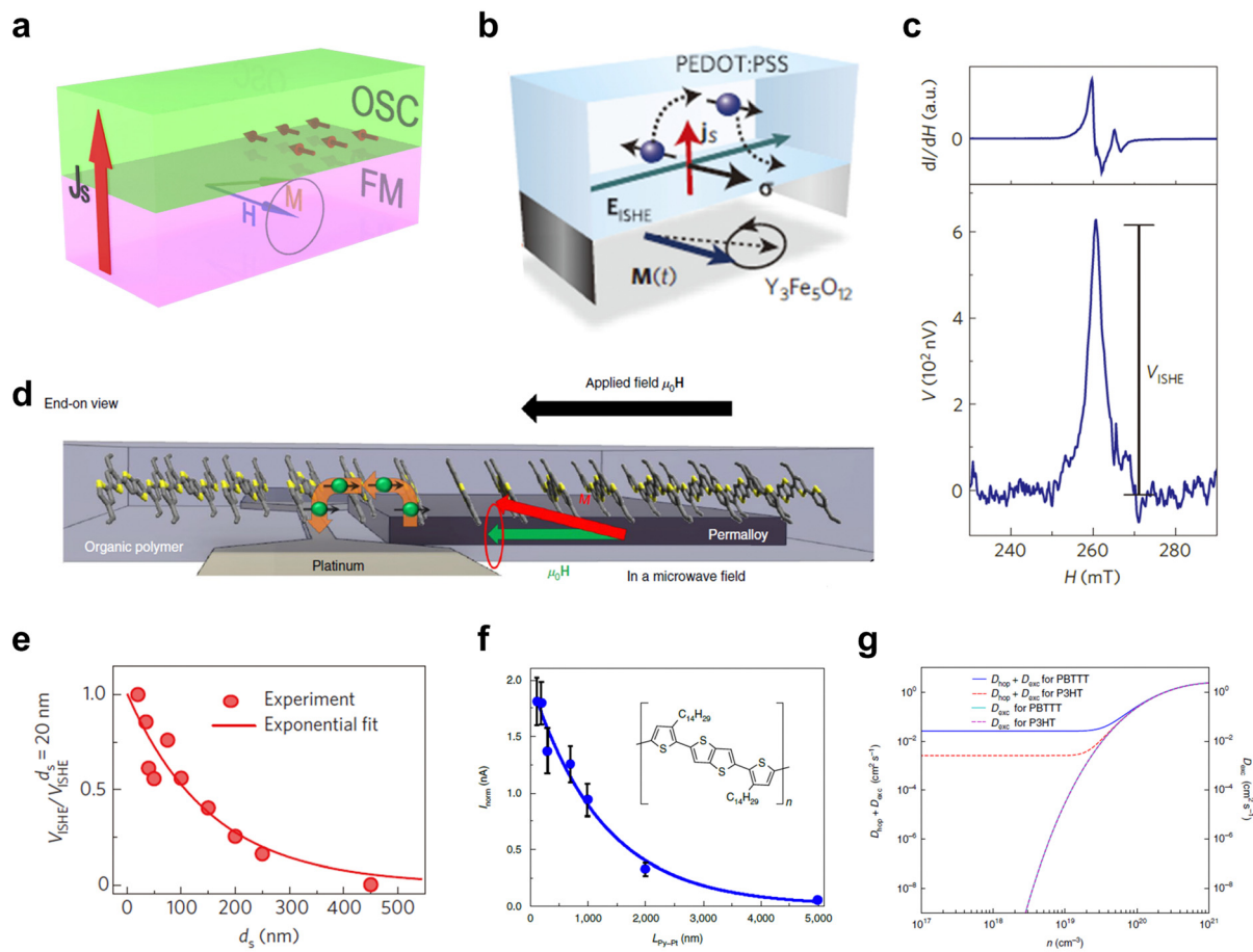
Fig. 5 (a) Schematic illustration of spin pumping, showing a spin current injected from the FM into the OSC at ferromagnetic resonance. (b) Operating principle based on spin pumping and ISHE in the bilayer device with a structure of Y_3Fe_5O_{12} /PEDOT:PSS. (c) Microwave absorption (ferromagnetic resonance signal dI/dH versus field H ) and the voltage spectra measured at 20 mV microwave excitation. (b and c) Reproduced with permission from ref. 112. Copyright 2013, Nature Publishing Group. (d) Illustrations of spin-current injection, transport, and detection in the spin pumping device with a trilayer architecture. (e) Thickness dependence of the normalized ISHE voltage for a vertical Ni_{80}Fe_{20} /PBTTT/Pt device. Reproduced with permission from ref. 109. Copyright 2014, Nature Publishing Group. (f) The thickness dependence of ISHE-induced current for a lateral device with a structure of Ni_{80}Fe_{20} /F4TCNQ-doped PBTTT/Pt. (g) Theoretical modeling of the diffusion coefficient as a function of the carrier density for PBDBTT and P3HT. (d, f and g) Reproduced with permission from ref. 117. Copyright 2019, Nature Publishing Group.
