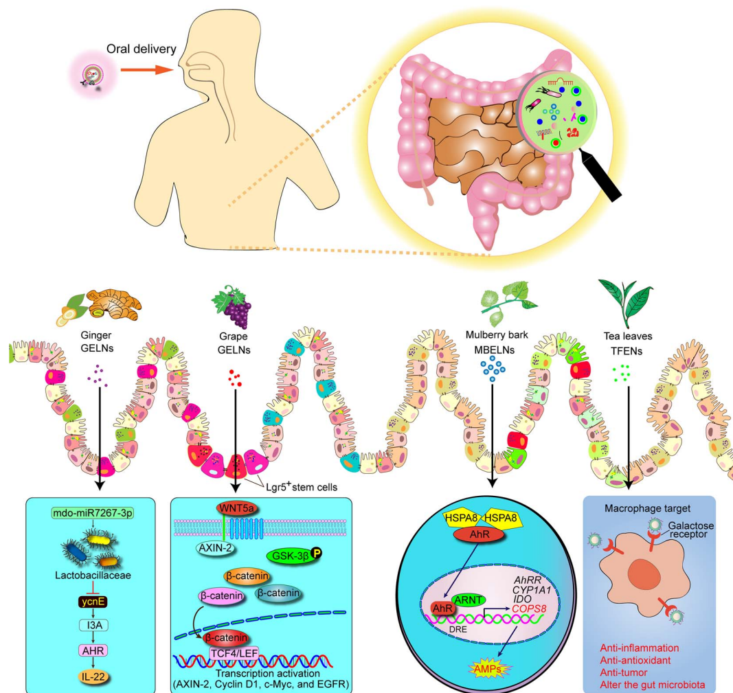
Fig. 3 Schematic representation of mechanism of PDEs that protects against colitis. AMP, anti-microbial peptides.
