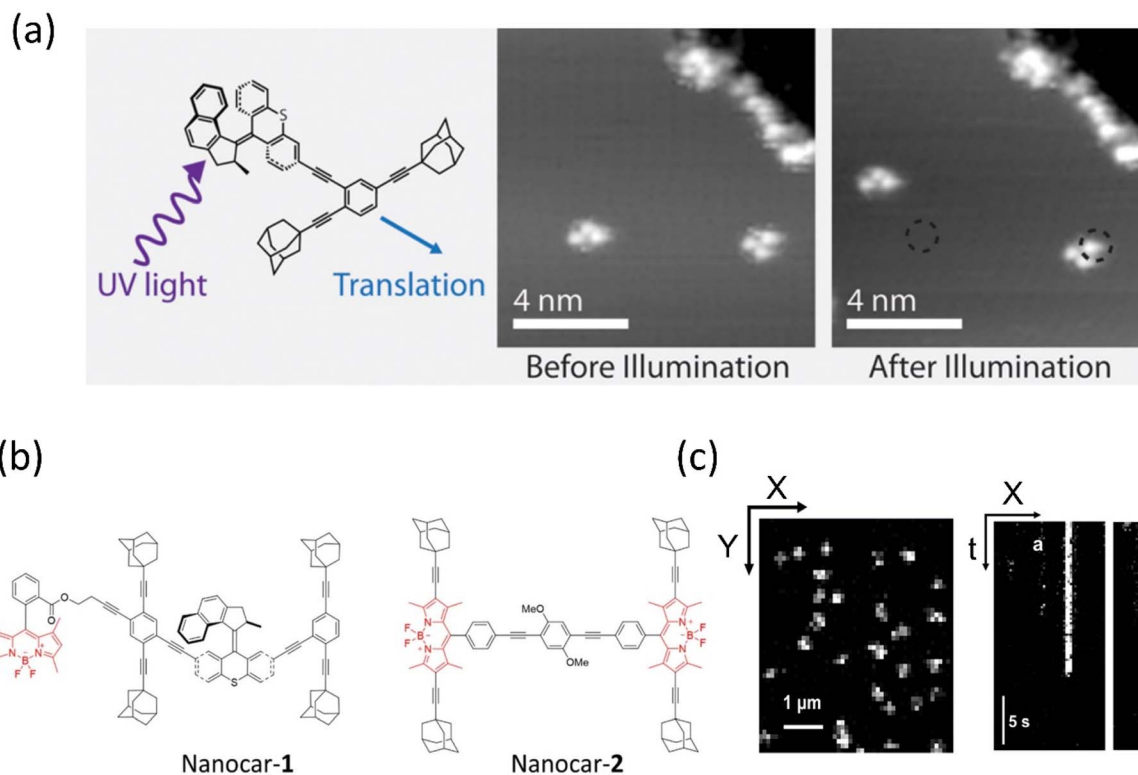
Fig. 6 (a) Molecular structure of light-activated motorized nanocar. The photoinduced motion of a molecular rotor on Cu(111) surface at 161 K. Reproduced with permission. 125 Copyright 2016, American Chemical Society. Line-scan imaging protocol (b) nanocar 1 & 2 equipped with adamantane wheels and BODIPY. (c) Conventional 2D photograph of nanocar 2 on the air-glass interface. (a and b) The line-scan images of nanocar 1 and 2 where nanocar 2 is in motion while nanocar 1 is immobilized. Reproduced with permission. 126 Copyright 2018, American Chemical Society.
