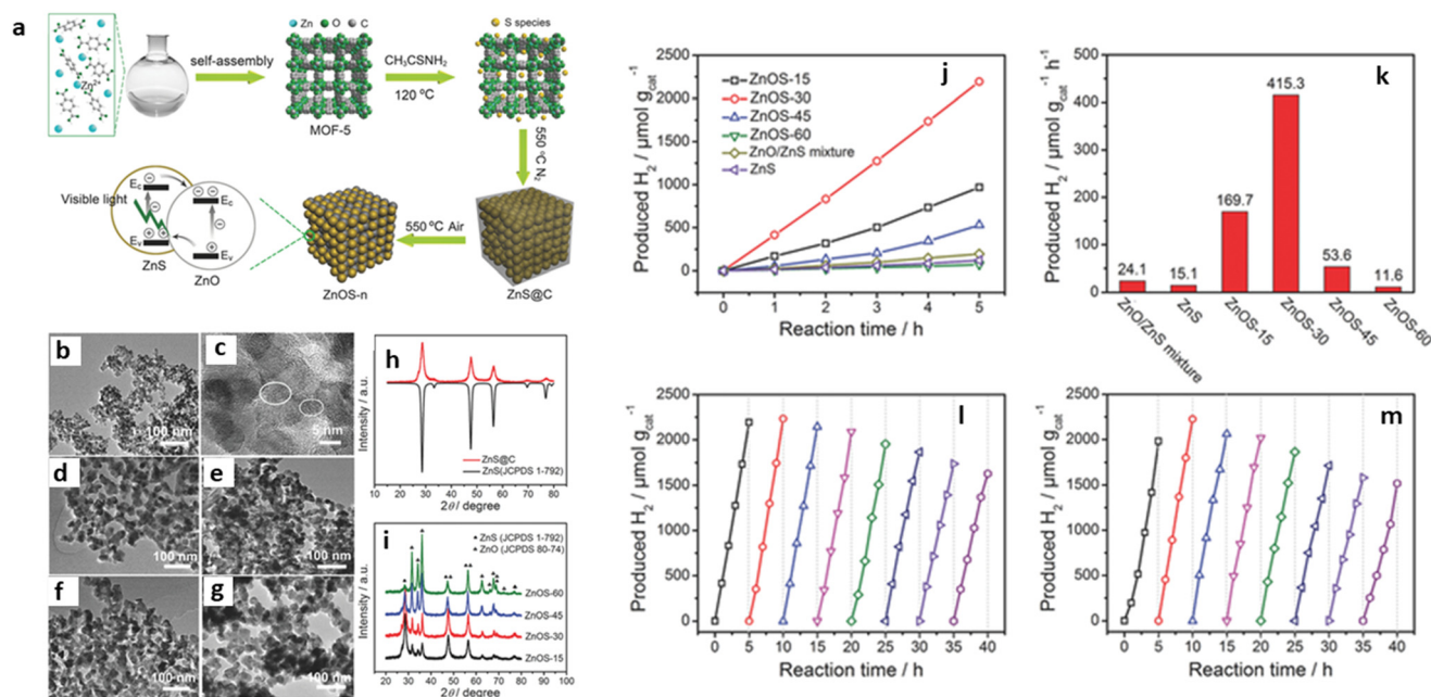
Fig. 8 (a) Schematic illustration of the synthetic procedure of ZnO/ZnS heterostructures. (b) TEM image, (c) HRTEM image, (d) ZnOS-15, (e) ZnOS-30, (f) ZnOS-45, and (g) ZnOS-60. (h) PXR D of ZnS@C. TEM images of (i) PXR D patterns of ZnOS- n . The photocatalytic performance of ZnO/ZnS heterostructures. (j) Time-dependent photocatalytic hydrogen evolution under visible-light irradiation ( \lambda > 420 nm, 300 W Xe lamp) for ZnOS- n . (k) Comparison of photocatalytic HER of ZnS/ZnO mixture, ZnS, and ZnOS- n under visible-light irradiation (evacuation every 5 h) for ZnOS-30 under visible-light irradiation. (l) Cycling test of H 2 evolution (evacuation every 5 h) for ZnOS-30 under visible-light irradiation. (m) Cycling test of H 2 evolution (evacuation every 5 h) for recycled and reprocessed ZnOS-30 after 40 h cycling test. 59
