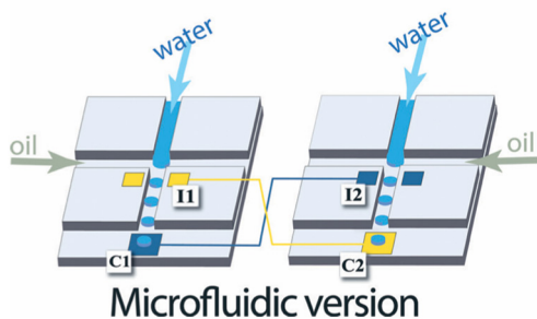
Classical Kelvin water dropper
