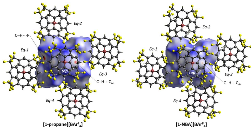
Fig. 3 Hirshfeld surfaces mapped over d_{\text{norm}} for [1\text{-NBA}]^+ and [1\text{-propane}]^+ within the octahedral arrays of neighbouring [\text{BARF}_4]^- anions with the anion labelling system indicated. Views are taken from above the 'top' anion looking down the \text{B}_{\text{top}} \cdots \text{Rh} \cdots \text{B}_{\text{bottom}} axis; the 'bottom' anion is obscured by the cation surface.
