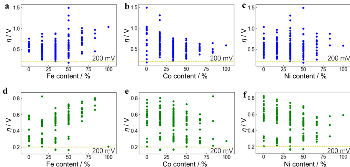
Fig. 4 Relationship between OER activity and Fe, Co, Ni contents. DFT-calculated OER overpotential ( \eta ) on Fe, Co, Ni-ternary \text{MO}_2 (a)–(c) and \text{M}(\text{OH})_2 (d)–(f) active sites vs. Fe, Co, Ni content from the site structure, respectively, as two-dimensional expansions of Fig. 3c and f. Under the same Fe, Co, or Ni content, the other two components can have different proportions, resulting in different overpotentials, so a series of points with a wide distribution is formed. The position where \eta is 200 mV is indicated by the yellow dotted lines, and the dots below them are regarded as active-site structures with high OER activity.
