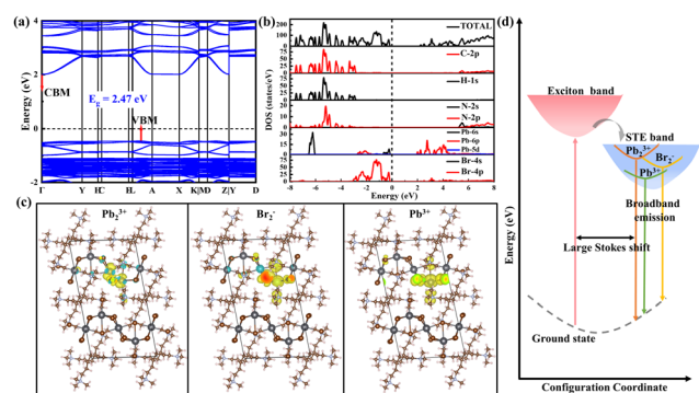
Fig. 4 (a) Calculated electronic band structures and (b) DOS of (HM)Pb 2 Br 6 . (c) Calculated charge density for (HM)Pb 2 Br 6 (Pb 2 3+ STLHs, Br 2 - and Pb 3 + STLHs holes) upon crystal lattice perturbation via the Pb–Pb, Br–Br and Pb–Br distances shortening. (d) Configuration coordinate diagram illustrating the luminescence mechanism.
