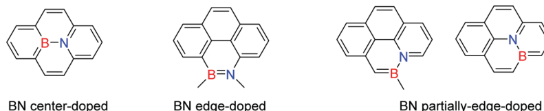
Fig. 1 The terminology of different locations of the BN unit in this review.
