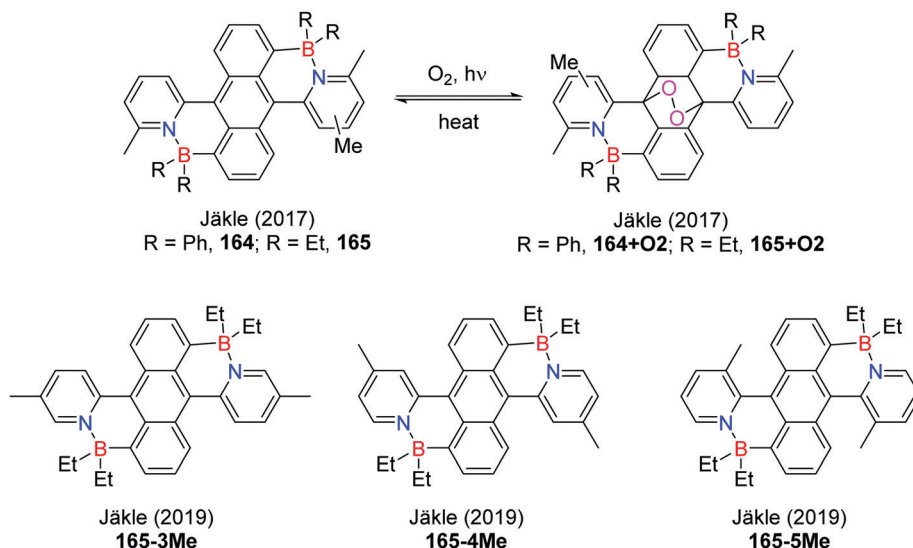
Fig. 50 Doubly BN-fused anthracenes for singlet \text{O}_2 sensitization.
