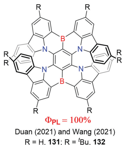
Fig. 39 Carbazole-based multi-BN-doped helicenes in different applications developed by Wang and Duan. Reprinted with permission from ref. 180. Copyright 2021 American Chemical Society.
