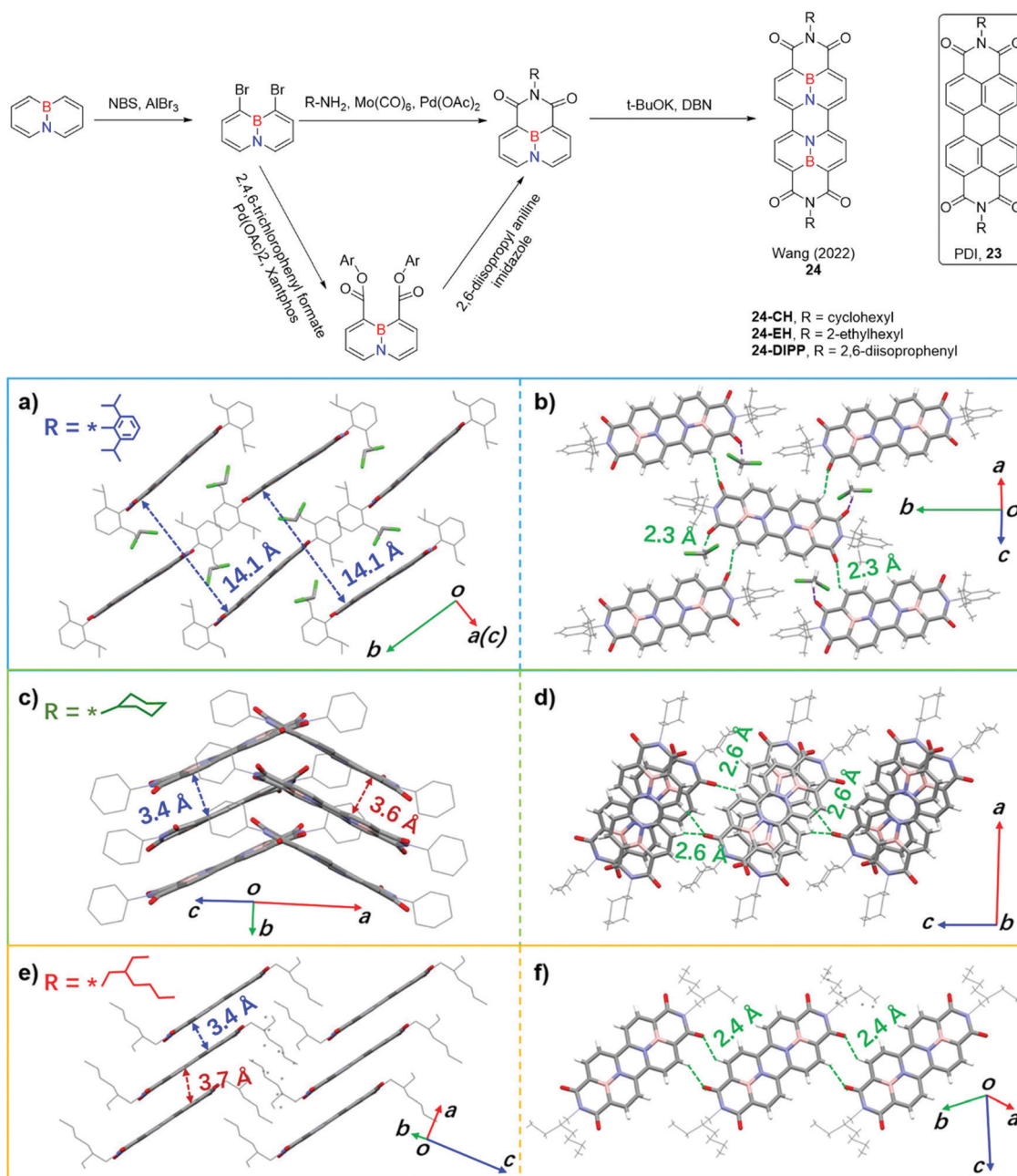
Fig. 7 Synthesis of (BN) 2 -PDIs, and crystal structures and packing motifs of 24 -DIPP (a and b), 24 -CH (c and d), and 24 -EH (e and f). Crystal structures of (a–f) reprinted with permission from ref. 71. Copyright 2022 American Chemical Society.
