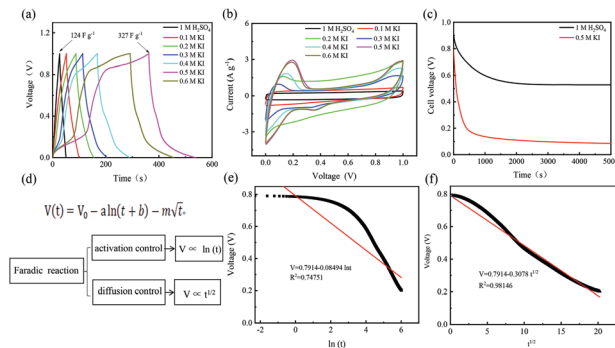
Fig. 3 Supercapacitors based on different KI content electrolytes (a) charge and discharge curves at various constant current densities of 1 \text{ A g}^{-1} . (b) Cyclic voltammetry curves at 10 \text{ mV s}^{-1} scan speed. (c) SDC curves were recorded after the device was charged to 1 \text{ V} at 1 \text{ A g}^{-1} constant current density. (d) The relationship between potential and time, independent variable \ln(t) or t^{1/2} . Supercapacitor SDC curve with 1.0 \text{ M H}_2\text{SO}_4 and 0.5 \text{ M KI} mixture electrolyte. (e) Fitting result of V and \ln(t) . (f) Fitting result of V and t^{1/2} .
