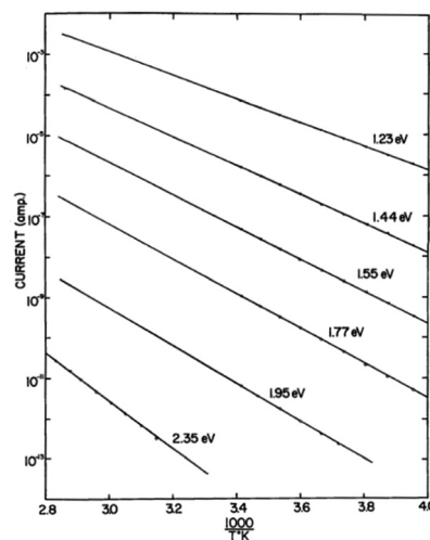
Fig. 3 Current vs. 1/T plots for crystalline haemoglobin for variously hydrated samples. Dry sample is the bottom curve. Copyright (1969) Wiley. Used with permission from B. Rosenberg and E. Postow, Ann. N. Y. Acad. Sci. , 1969, 158 , 161–190. 17 © 1969 John Wiley & Sons, Inc.
