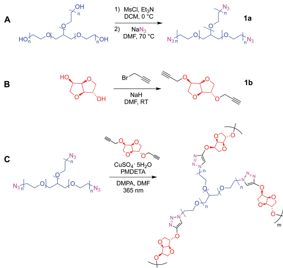
Scheme 1 Synthetic protocols employed in the preparation of (A) triazide glycerol ethoxylate and (B) bis-alkyne isosorbide derivatives. (C) Synthesis of hydrogel films via \text{Cu(I)} mediated photo-click reaction.
