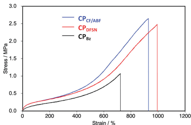
Fig. 5 Stress–strain curves of \text{CP}_{\text{CF/ABF}} (blue), \text{CP}_{\text{DFSN}} (red) and \text{CP}_{\text{Bz}} (black) films (100 mm \text{min}^{-1} , 30 °C).
