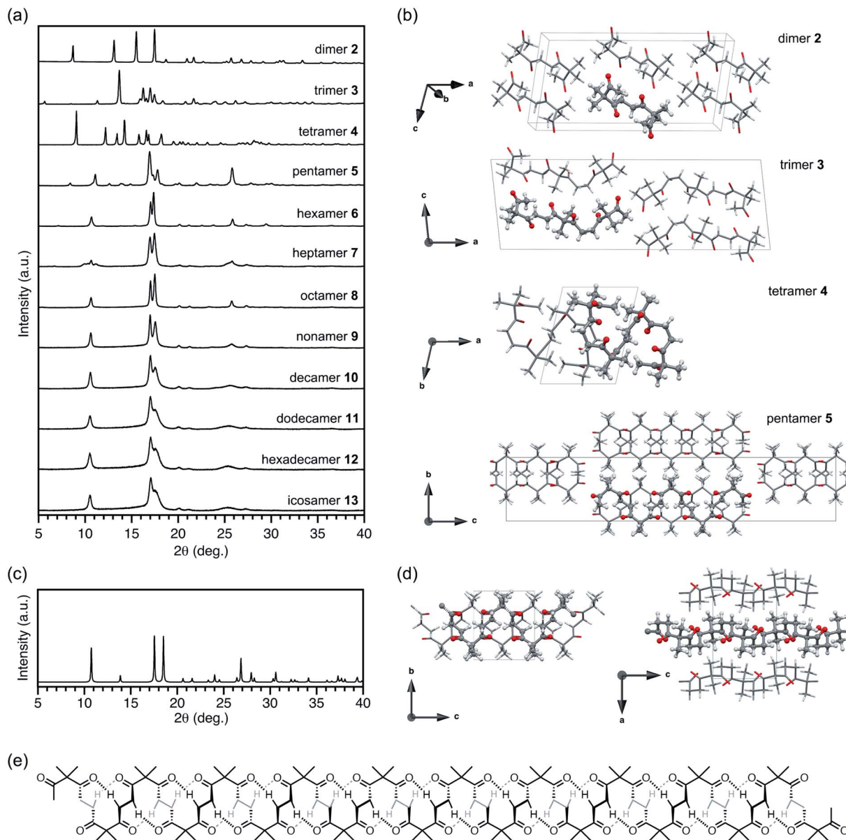
Fig. 2 (a) PXR patterns of discrete oligomers 2–13. (b) Conformations and packing structures of 2–5 obtained by SCXRD analysis. (c) Simulated PXR pattern of the energy minimized crystal structure of infinite polyketones. (d) Energy minimized packing structure of infinite polyketone crystals. (e) Chemical structure of icosamer 13 in the helical conformation.
