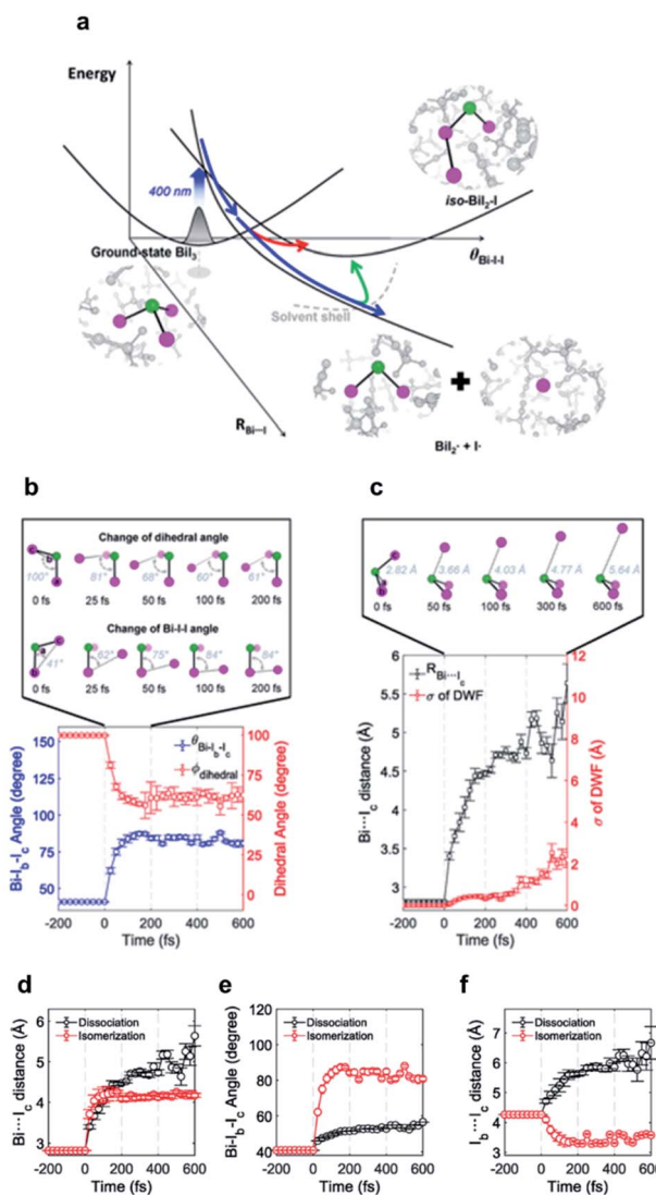
Fig. 3 (a) Schematic representation of the photodynamics of \text{BiI}_3 in acetonitrile. (b) Changes of the \text{Bi-1}_b\text{-1}_c angle and \text{I}_a\text{-Bi-1}_b\text{-1}_c dihedral angle during the roaming-mediated isomerization determined from structural analysis on the fs-TRXL data for \text{BiI}_3 in acetonitrile. (c) Changes of the \text{Bi}\cdots\text{I}_c distance and the root-mean-squared displacement ( \sigma ) associated with the pair distances containing \text{I}_c . Insets in (b) and (c) show transient structures at representative time delays. (d-f) Comparison of the structural motions for the dissociation and roaming-mediated isomerization channels through (d) \text{Bi}\cdots\text{I}_c distance, (e) \text{Bi-1}_b\text{-1}_c angle, and (f) \text{I}_b\cdots\text{I}_c distance. Reproduced from ref. 65 with the permission of Springer Nature, copyright 2021.
