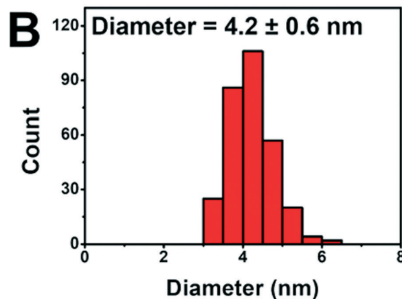
Fig. 6 A. TEM micrograph and B. NP size distribution at 1.4 mM metal and 1 mM PEGSH.
