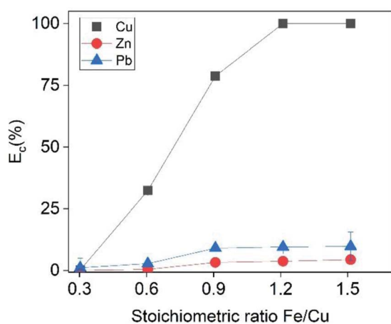
Fig. 5 Cementation efficiency of Cu as a function of the stoichiometric ratio Fe/Cu. Conditions: t = 30 min, [Cu]_i = 500 mmol L -1 , [Zn]_i = 23 mmol L -1 , [Pb]_i = 23 mmol L -1 .
