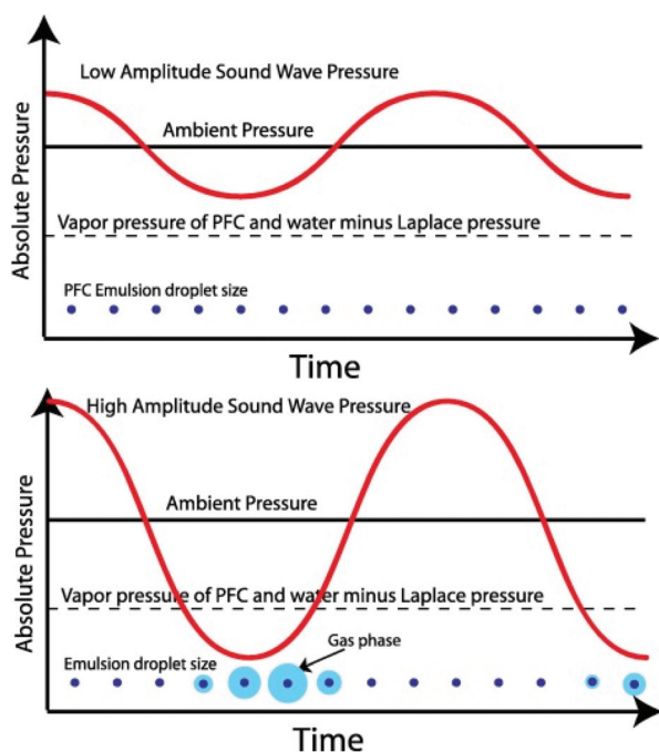
Fig. 2 Schematic of an ultrasonic acoustic wave in a perfluorocarbon emulsion. The graphs show emulsion droplets (not to scale) that only vaporise into the gas phase when the acoustic pressure is below the Laplace pressure 37 (this figure has been reproduced from ref. 37 with permission from Elsevier, copyright 2014).
