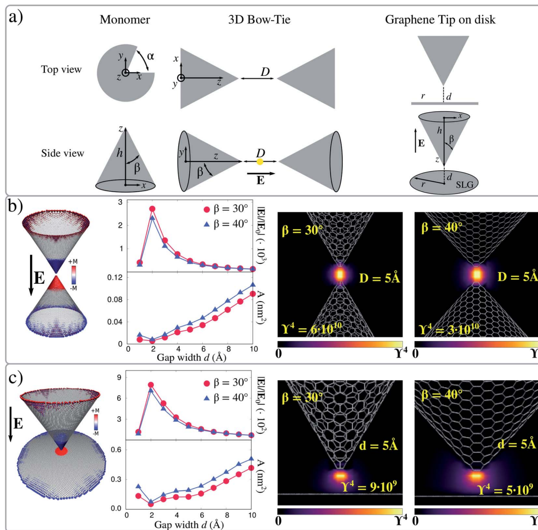
Fig. 3 (a) Geometrical parameters of graphene-based nanocones, 3D bow-ties and graphene tip-disks. (b) 3D bow-tie electric field enhancement factors ( |E|/|E_0| and Y^4 ) and localization area ( A ) for both \beta = 30^\circ and \beta = 40^\circ , as a function of the gap width ( D ) calculated at the boundary dipolar plasmon (see left panel) in the center of the gap. \beta = 30^\circ and \beta = 40^\circ electric field enhancement factors color map for 3D bow-tie nanostructure with D = 5 \text{ \AA} . (c) Graphene tip-disk electric field enhancement factors ( |E|/|E_0| and Y^4 ) and localization area ( A ) for both \beta = 30^\circ and \beta = 40^\circ , as a function of the gap width ( d ) calculated at the boundary dipolar plasmon (see left panel) in the center of the gap. \beta = 30^\circ and \beta = 40^\circ electric field enhancement factors color maps for graphene tip-disk nanostructure with d = 5 \text{ \AA} . The Fermi level is set to E_F = 0.4 \text{ eV} for each configuration.
