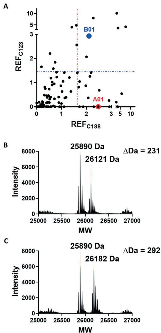
Fig. 2 Acrylamide fragment screening against fRab27A-C123 and fRab27A-C188. A ) 2D scatter plot of REF values against fRab27A-C123 (Y-axis) and fRab27A-C188 (X-axis) for 126-fragment library screened in the qIT assay. Hits were defined as REF values over one standard deviation from the median value, shown by a dotted line (in blue for fRab27A-C123, in red for fRab27A-C188). Selected hits A01 for fRab27A-C188 (red) and B01 for fRab27A-C123 (blue), are highlighted. B ) Intact protein mass spectrometry for the fRab27A-C188- A01 adduct shows the expected mass shift (24 h incubation at 4 °C). C ) Intact protein mass spectrometry for fRab27A-C123- B01 shows the expected mass shift (8 h incubation at 4 °C).
