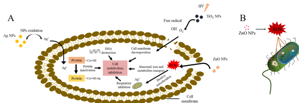
Fig. 3 Antimicrobial mechanisms of metal and metallic oxide nanoparticles. (A) Antimicrobial mechanism of metal nanoparticles ( \text{Ag}^+ ) and metallic oxide nanoparticles ( \text{TiO}_2 , \text{ZnO} ). (B) The antibacterial mechanism of \text{ZnO} . (1) Disruption the plasma membrane permeability to make some substances flow out; (2) inhibition of DNA replication; (3) protein denaturation.
