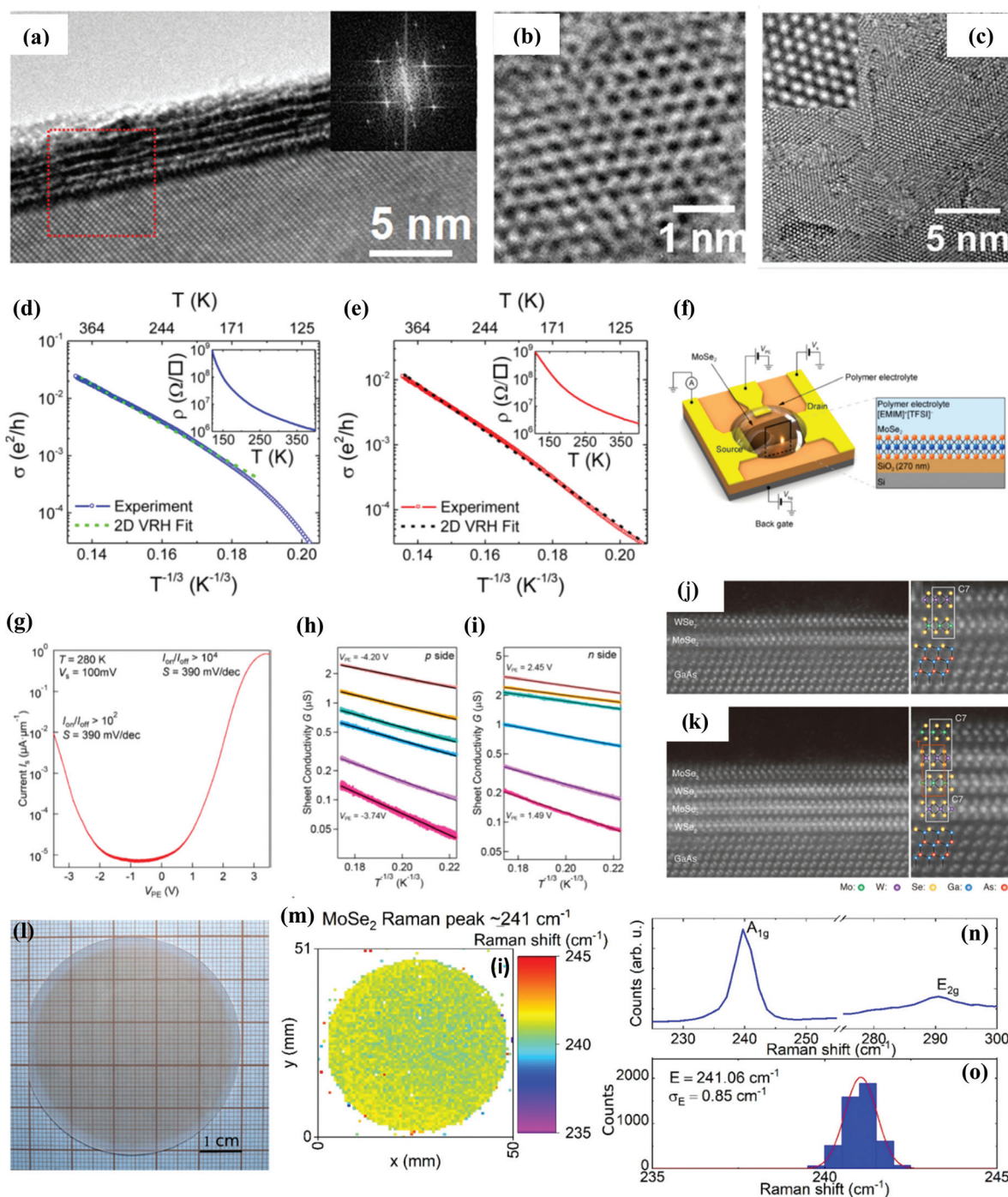
Fig. 3 (a) HR-STEM image of a layered structure of MoTe 2 . Inset shows the fast Fourier transform (FFT) of the area marked by the red square. The plan-view TEM image depicts the hexagonal arrangement of atoms in the (b) MoTe 2 thin film and (c) MoSe 2 lattice. Inset shows the zoomed-in view for 2 \times 2 \text{ nm}^2 . Electrical transport measurements show the conductivity variation with T^{-1/3} for (d) MoTe 2 and (e) MoSe 2 . Insets of (d, e) show the variations of the measured resistivities with temperature. The figures have been reproduced from ref. 67. (f) The schematic device structure of the MoSe 2 thin film-based EDLT. (g) Variation of the channel current with polymer electrolyte voltage (VPE) depicting ambipolar behavior. (h and i) Sheet conductivity ( G_{\text{SH}} ) as a function of T^{-1/3} on the p and n sides for different values of V_{\text{PE}} . The figure has been reproduced from ref. 45. The HAADF-STEM images for the (j) bilayered WSe 2 /MoSe 2 and (k) four-layered MoSe 2 /WSe 2 heterostructures grown on GaAs(111)B. The figure has been reproduced from ref. 71. (l) Optical image of epitaxially grown MoSe 2 . (m) Peak energy of the A 1g mode obtained through Raman mapping. (n) Typical Raman spectrum of MoSe 2 . (o) Distribution of the peak energy of the A 1g mode indicating the mean value and standard deviation. The figure has been reproduced from ref. 73.
