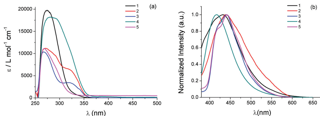
Fig. 2 (a) UV-Vis electronic absorption spectra and (b) emission spectra (excitation at 320 nm) of 1–5 in DMSO solutions ( \sim 5 \times 10^{-5}\text{ M} ).
