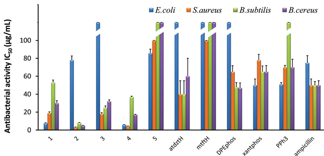
Fig. 3 In vitro antibacterial activity of 1–5, and their ligands atdztH, mtftH, DPEphos, xantphos, and PPh 3 in free form, expressed as half-minimum inhibitory concentration (IC 50 ) values ( \mu\text{g mL}^{-1} ) provided by a nonlinear curve fit-growth/sigmoidal-dose response on the experimental optical density data. Values are expressed as mean \pm standard deviation (SD) of three replicate measurements (with the exception of values higher than 100 \mu\text{g mL}^{-1} ).
