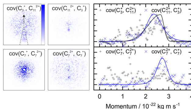
Fig. 4 Left: The covariance map images for dissociation of PHE 3+ into \text{C}_3\text{H}_x^{+} and \text{C}_{11}\text{H}_y^{2+} , and \text{C}_7\text{H}_x^{+} and \text{C}_7\text{H}_y^{2+} , top and bottom, respectively. Nomenclature as in Fig. 2. Covariance signal in the \text{cov}(\text{C}_7^{+}, \text{C}_7^{2+}) image cannot be discerned above the noise level but the \text{cov}(\text{C}_7^{2+}, \text{C}_7^{+}) image provides the TKER for the dissociation process. The centre of the \text{cov}(\text{C}_7\text{H}_x^{+}, \text{C}_7\text{H}_y^{2+}) image shows detector saturation due to the flight times of \text{C}_7\text{H}_x^{+} and \text{C}_{14}\text{H}_y^{2+} overlapping. Right: the momentum profiles extracted from the corresponding covariance images using the region marked by dashed lines in the \text{cov}(\text{C}_3^{+}, \text{C}_{11}^{2+}) image. All images and momentum profiles are individually normalized.
