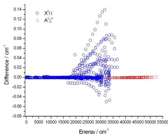
Fig. 3 Differences between the MARVEL energy levels of this study and the empirical results of MoLLIST 55 , 55 concerning the X^2\Pi and A^2\Sigma^+ electronic states of the ^{16}\text{OH} radical.
