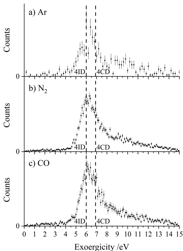
Fig. 3 Experimental exoergic distributions resulting from the CID channel \text{CH}_2\text{CN}^{2+} + \text{X} \rightarrow \text{CH}_2\text{N}^+ + \text{C}^+ + \text{X} , where X = (a) Ar, (b) \text{N}_2 , and (c) CO. Dashed lines are marked at 6.0 eV and 6.9 eV in each of the distributions to show the predicted literature exoergicities associated with the involvement of the quartet linear isocyanide dication 4ID and the cyclic quartet dication 4CD respectively. The error bars represent two standard deviations of the counts.
