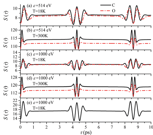
Fig. 11 The dependence of the temporal profile S(\tau) (30) on the ionization site n = C, O is defined by the recoil parameter \alpha_n k R_0 , where \alpha_C = 0.571 , \alpha_O = 0.429 . \theta = 0 . Panel (e) shows the sum S(\tau) = S_C(\tau) + S_O(\tau) , where S_C(\tau) and S_O(\tau) are the S(\tau) functions (30) for carbon and oxygen shown in the panel (c).
