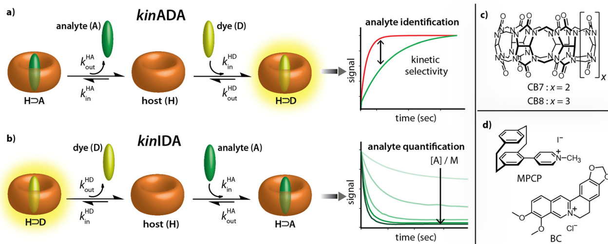
Fig. 2 (a and b) Working principle of the kinetic analyte displacement assay ( kinADA ) and kinetic indicator displacement assay ( kinIDA ). The kinetic parameters k_{\text{in}}^{\text{HA}} and k_{\text{out}}^{\text{HA}} describe the rate constants for association and dissociation of the \text{H} \rightarrow \text{A} complexes. Analogously, k_{\text{in}}^{\text{HD}} and k_{\text{out}}^{\text{HD}} refer to the kinetic parameters of the \text{H} \rightarrow \text{D} complex. (c and d) Chemical structures of the macrocycles CB7 and CB8 and the environment-sensitive fluorophores MPBP and BC utilized in this study as host (H) and indicator dyes (D), respectively.
