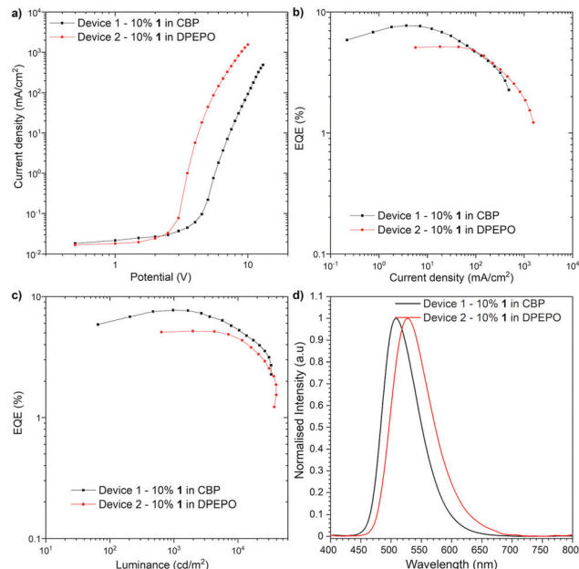
Fig. 4 Device characteristic.
