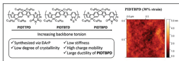
Fig. 9 Left panel: Chemical structures of PIDTTPD , PIDTBTD , and PIDTBPD along with the design features; right panel: surface morphology of PIDTBPD under 30% strain obtained using contact mode AFM. Reproduced with permission from American Chemical Society. 87
